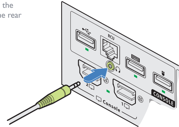
Connection to console speakers
