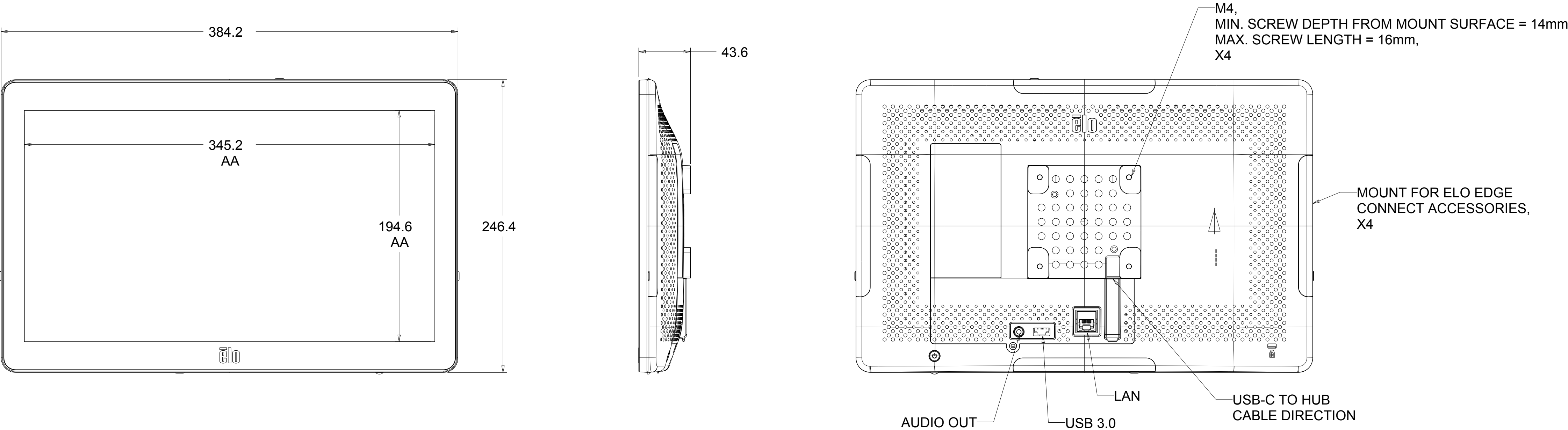
15.6" WITH HUB NOT ATTACHED TO BACK
