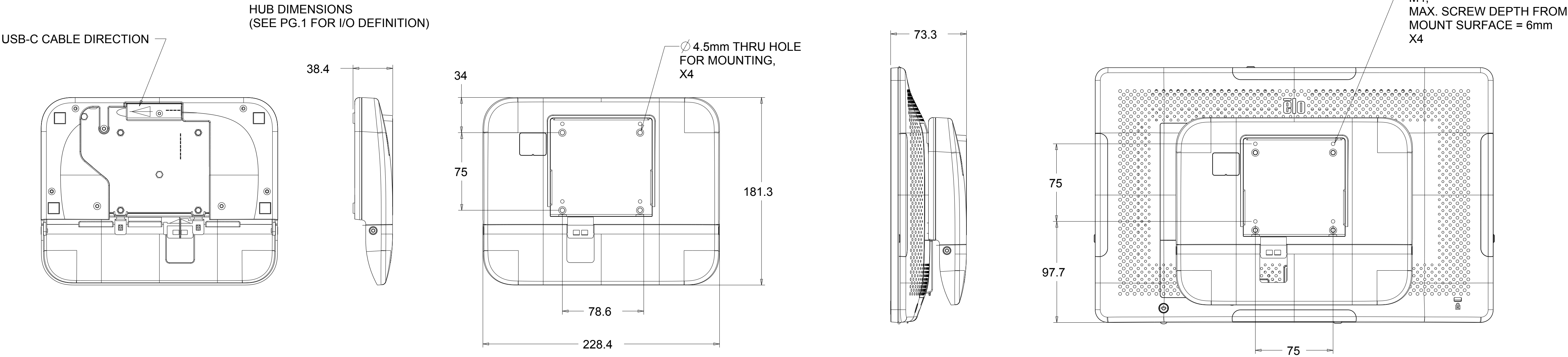
15.6" WITH HUB ATTACHED TO BACK
